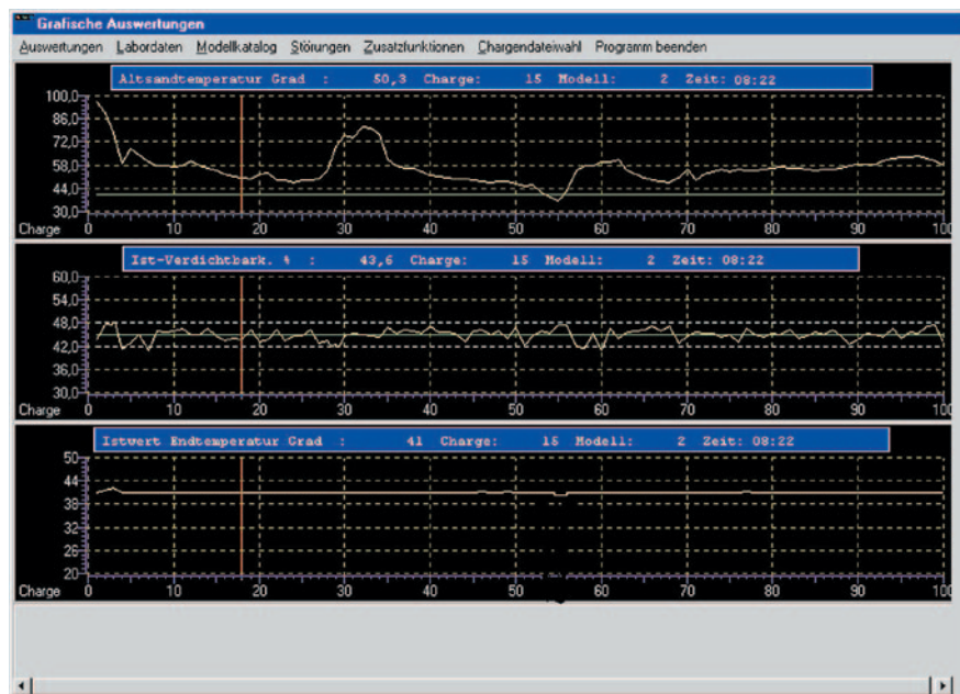
Fig. 8: SandExpert: View of the temperature curve of the return sand and the newly prepared molding material
